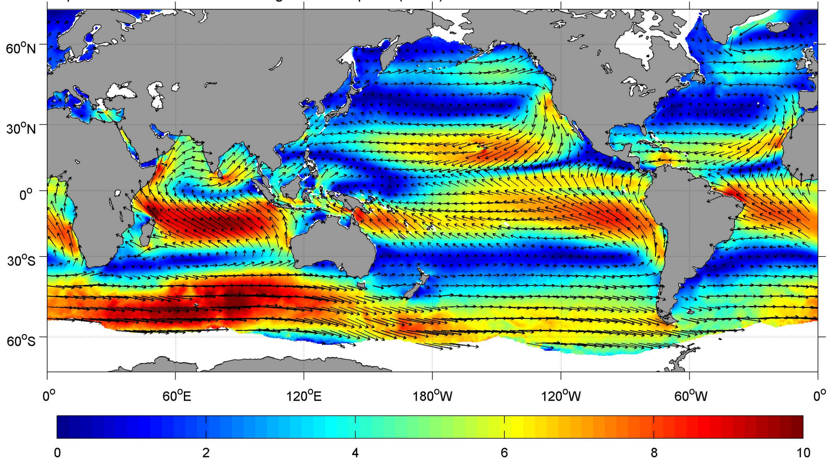
September SCOW Vector Averaged Wind Speed ( \text{m s}^{-1} ) and Direction
