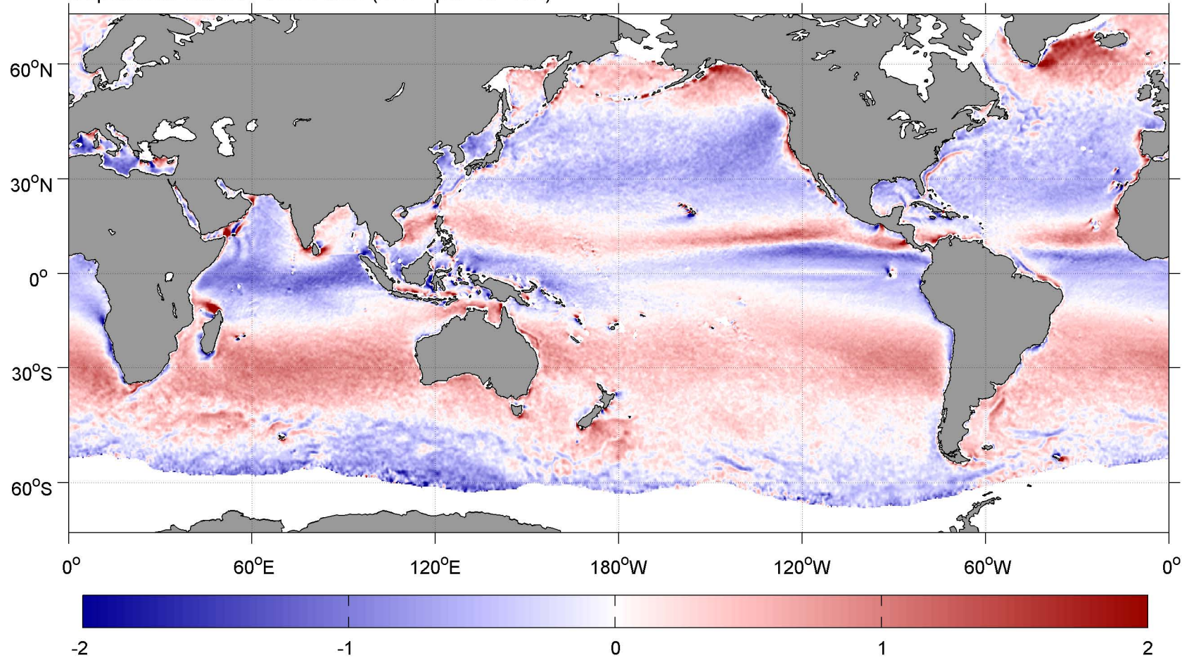
September SCOW Wind Curl ( \text{m s}^{-1} per 10^2 \text{ km} )
