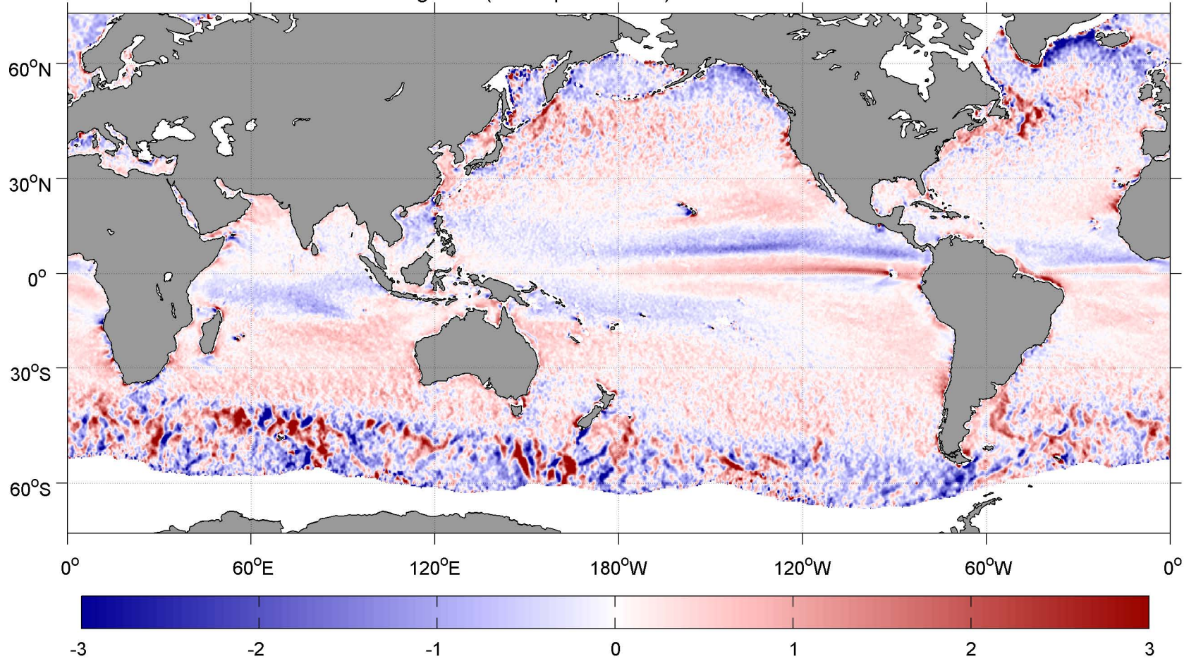
October SCOW Wind Stress Divergence ( \text{N m}^{-2} per 10^4 \text{ km}^2 )
