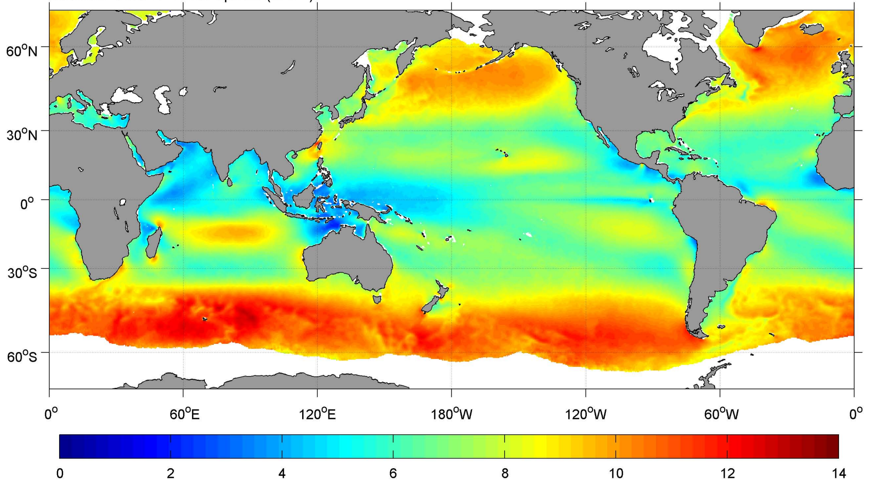
October SCOW Wind Speed ( \text{m s}^{-1} )
