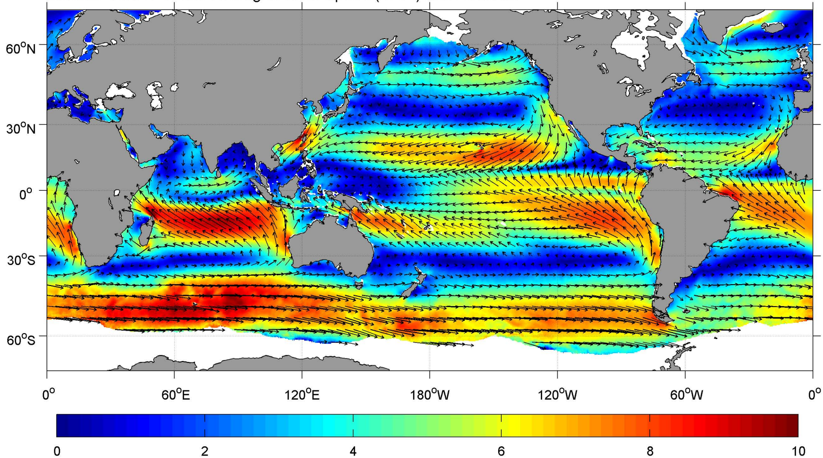
October SCOW Vector Averaged Wind Speed ( \text{m s}^{-1} ) and Direction
