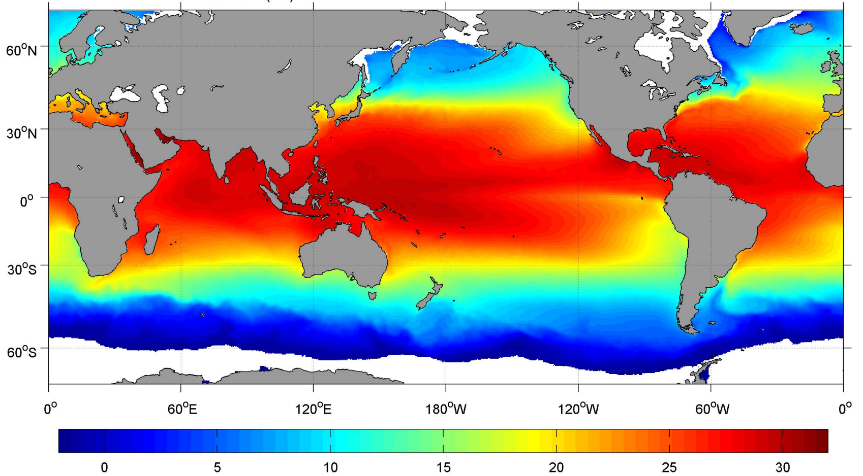
October SCOW AVHRR SST ( ^{\circ}\text{C} )
