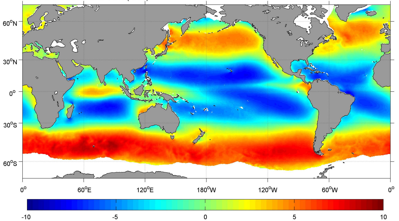
November SCOW Zonal Wind ( \text{m s}^{-1} )
