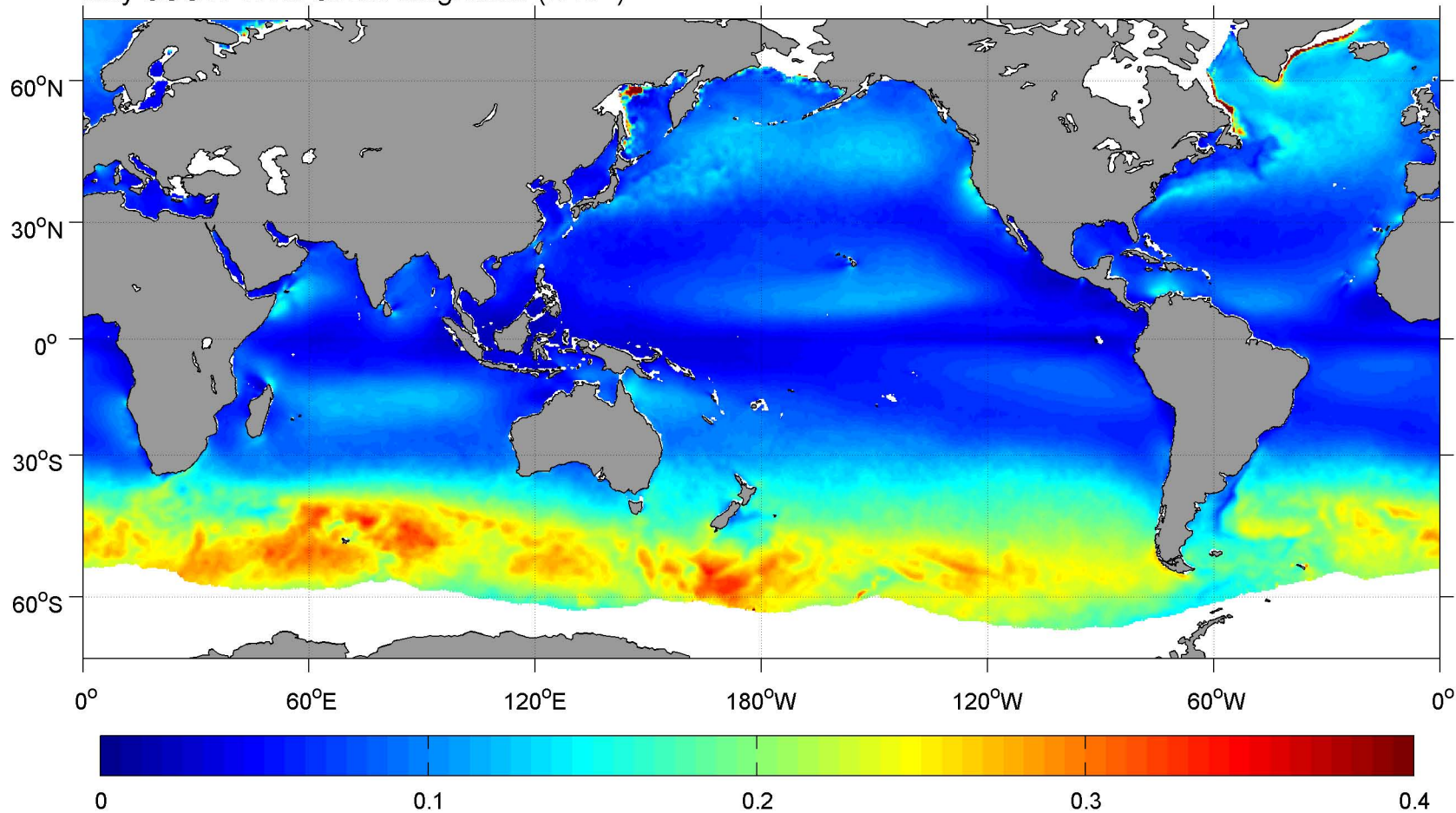
May SCOW Wind Stress Magnitude ( \text{N m}^{-2} )
