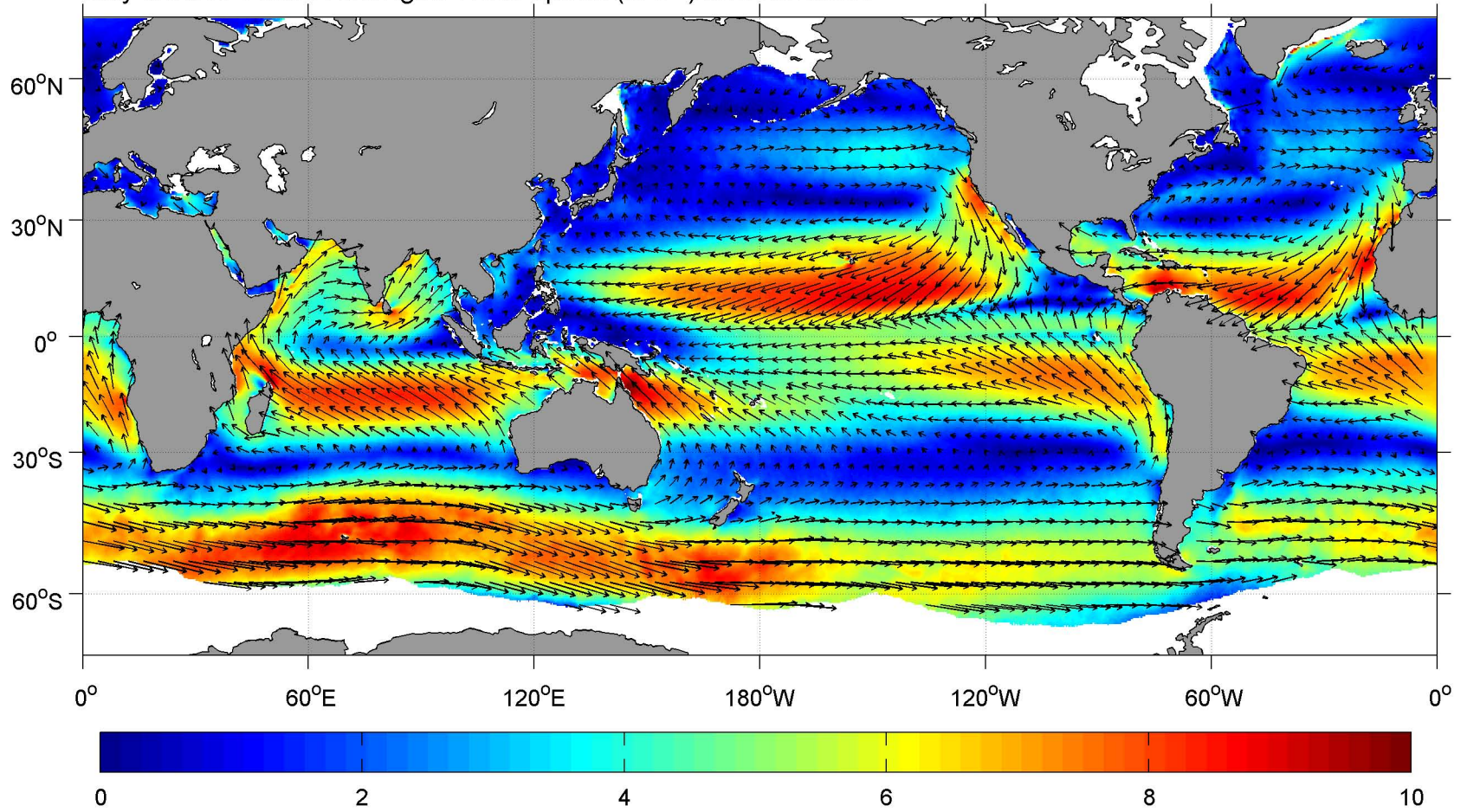
May SCOW Vector Averaged Wind Speed ( \text{m s}^{-1} ) and Direction
