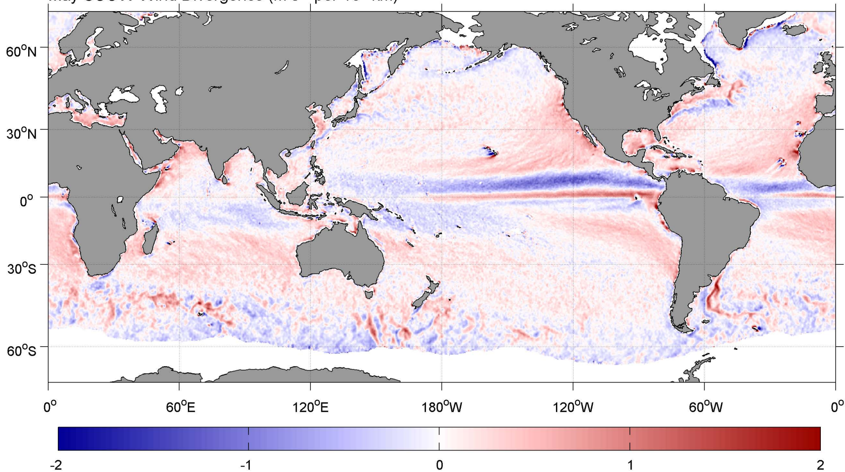
May SCOW Wind Divergence ( \text{m s}^{-1} per 10^2 \text{ km} )
