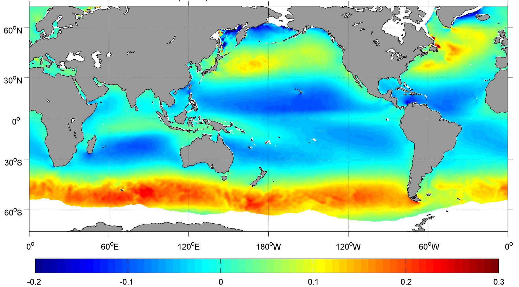
March SCOW Zonal Wind Stress ( \text{N m}^{-2} )
