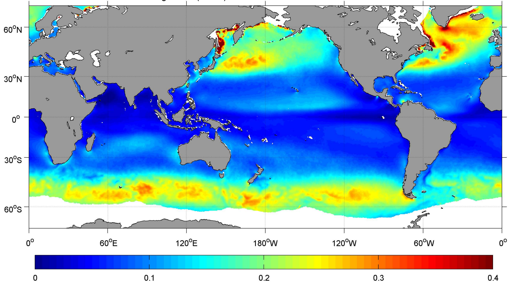
March SCOW Wind Stress Magnitude ( \text{N m}^{-2} )
