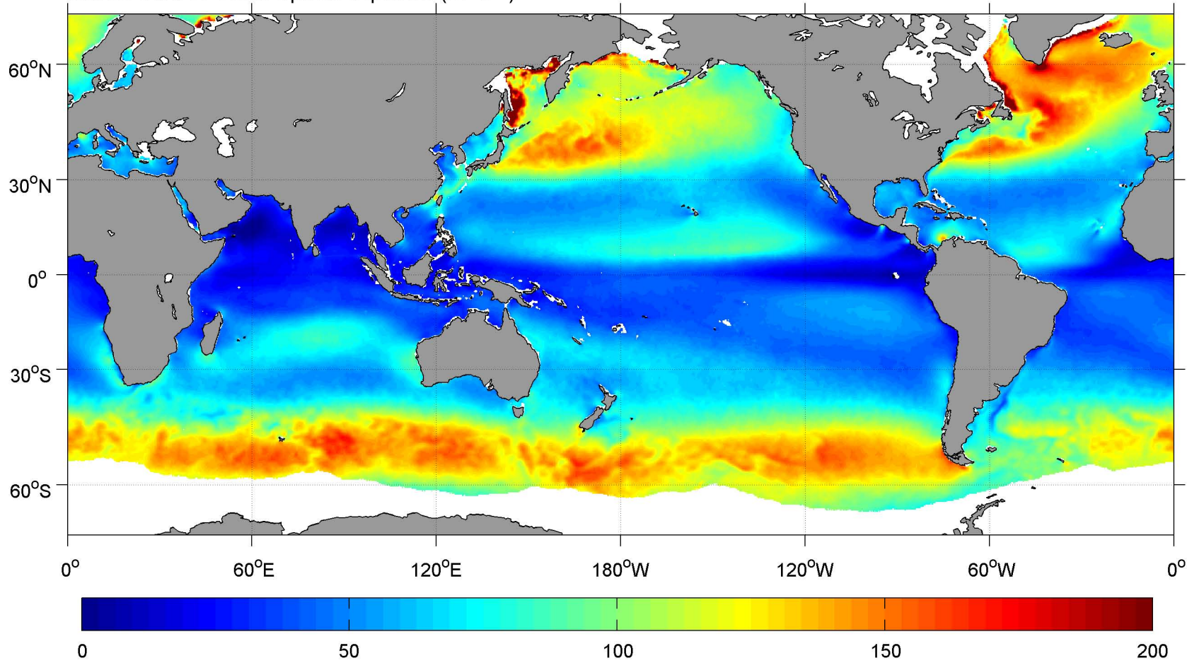
March SCOW Wind Speed Squared ( \text{m}^2 \text{s}^{-2} )
