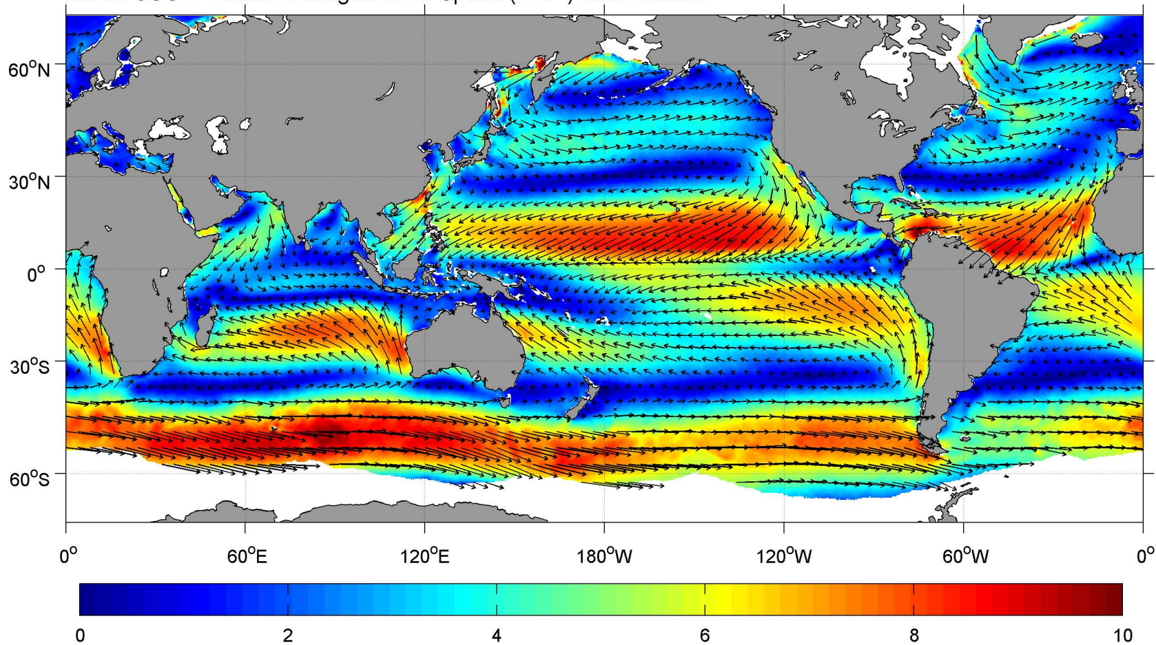
March SCOW Vector Averaged Wind Speed ( \text{m s}^{-1} ) and Direction
