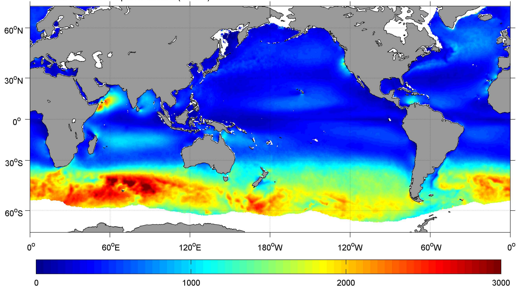
June SCOW Wind Speed Cubed ( \text{m}^3 \text{s}^{-3} )
