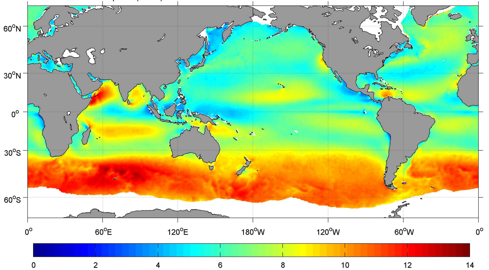
June SCOW Wind Speed ( \text{m s}^{-1} )
