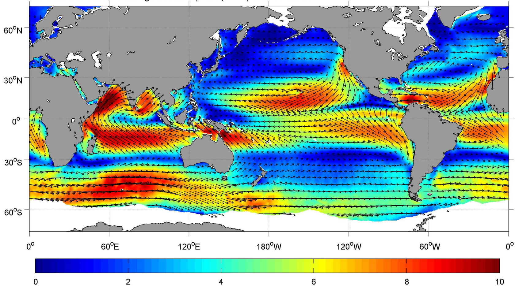
June SCOW Vector Averaged Wind Speed ( \text{m s}^{-1} ) and Direction
