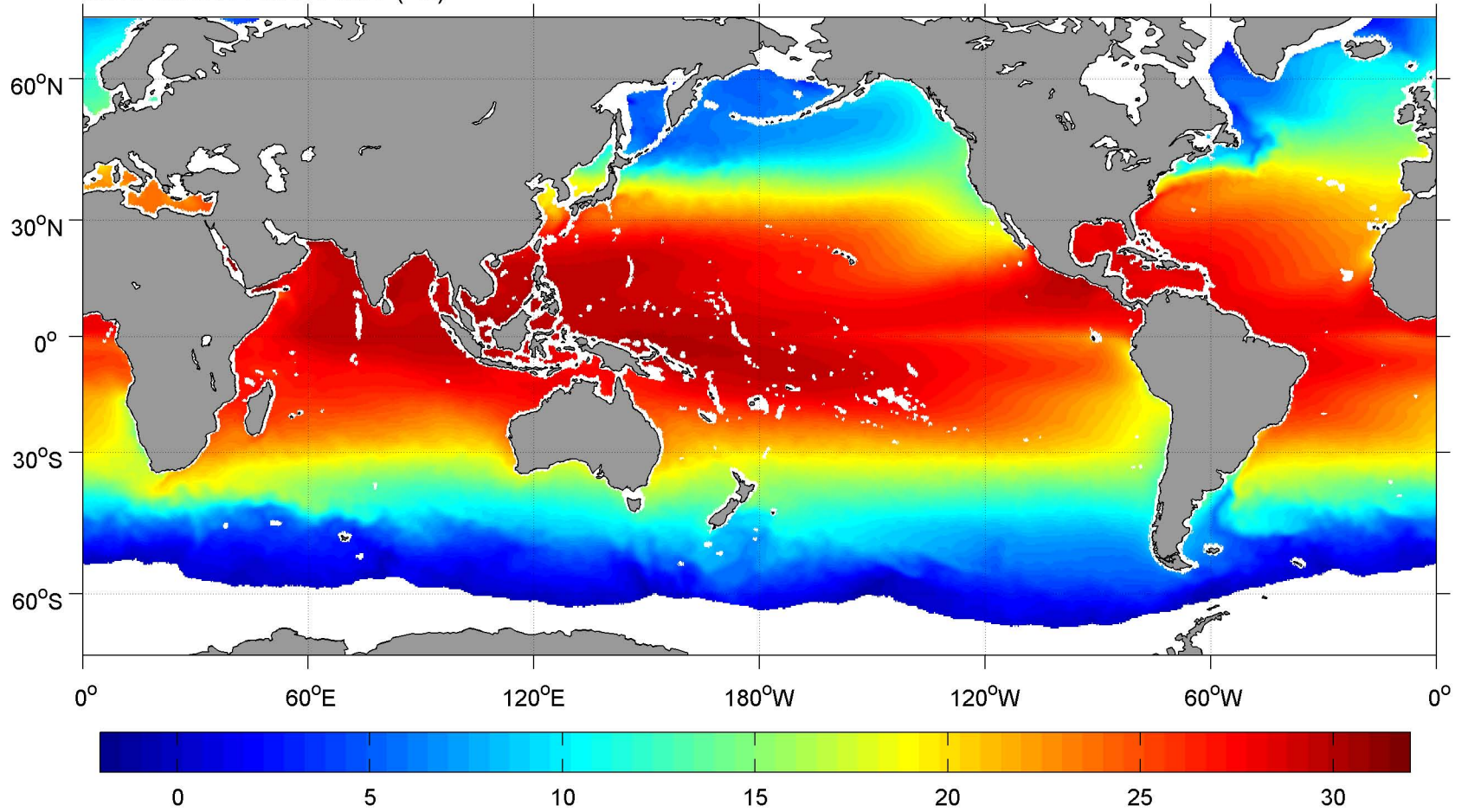
June SCOW AMSR SST ( ^{\circ}\text{C} )
