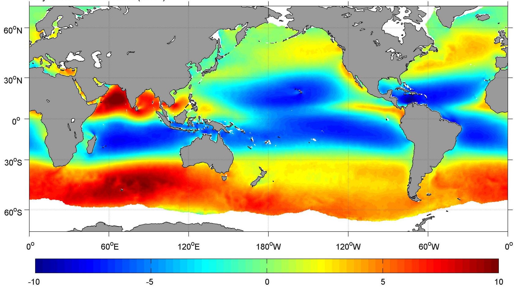
July SCOW Zonal Wind ( \text{m s}^{-1} )
