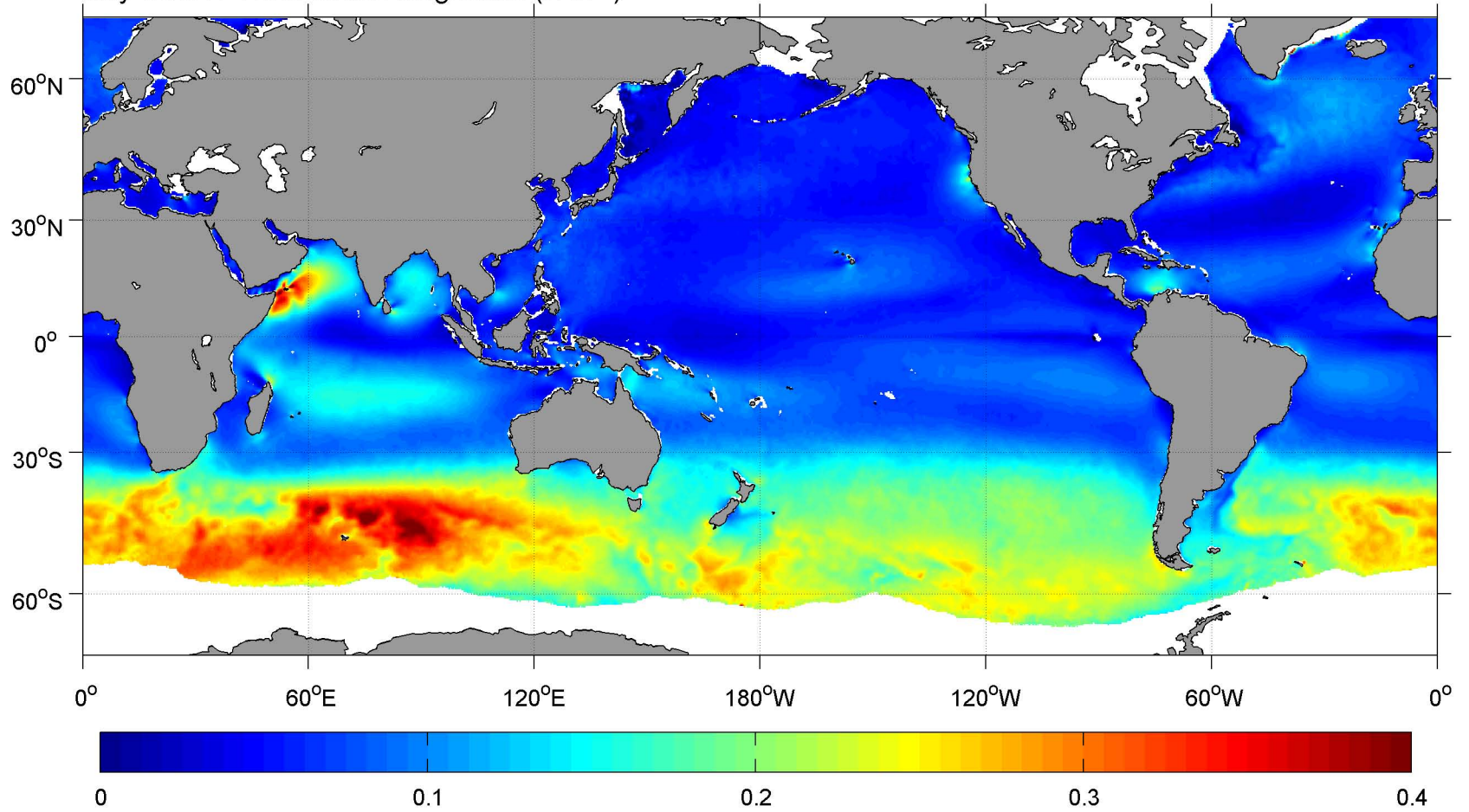
July SCOW Wind Stress Magnitude ( \text{N m}^{-2} )
