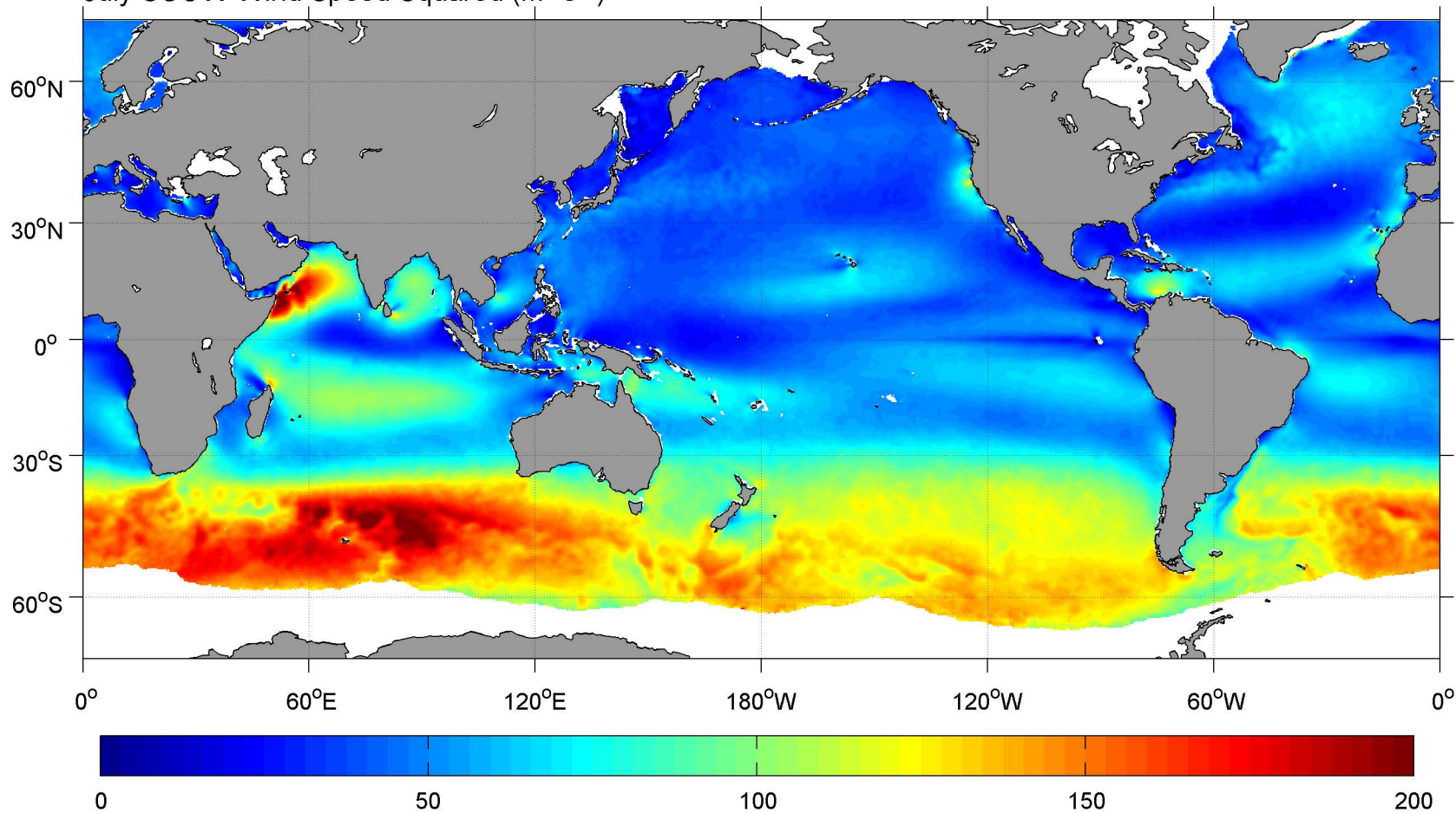
July SCOW Wind Speed Squared ( \text{m}^2 \text{s}^{-2} )
