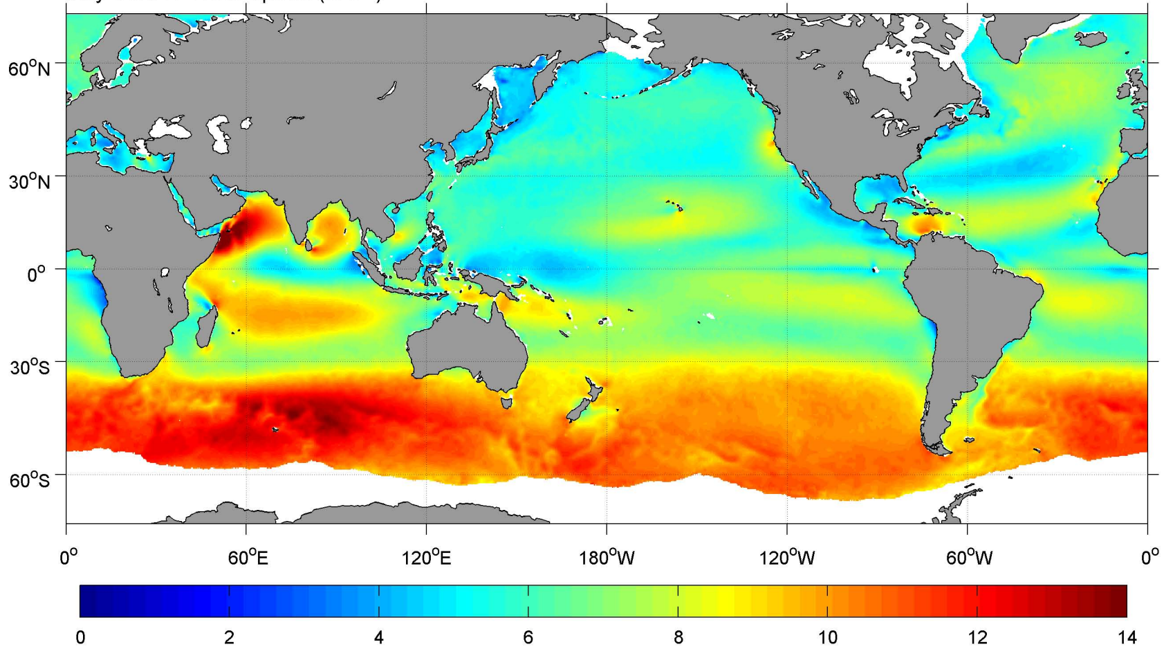
July SCOW Wind Speed ( \text{m s}^{-1} )
