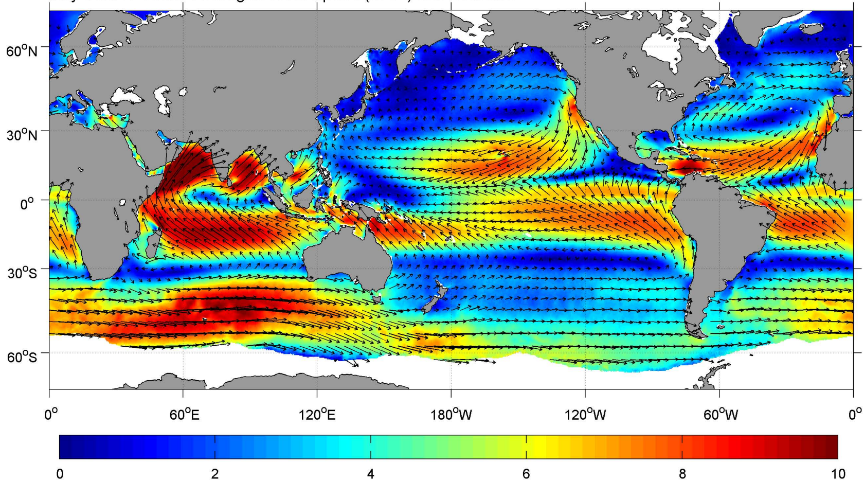
July SCOW Vector Averaged Wind Speed ( \text{m s}^{-1} ) and Direction
