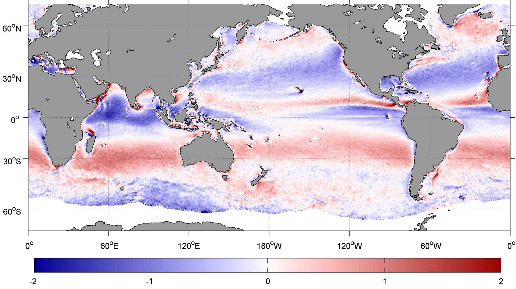
July SCOW Wind Curl ( \text{m s}^{-1} per 10^2 \text{ km} )
