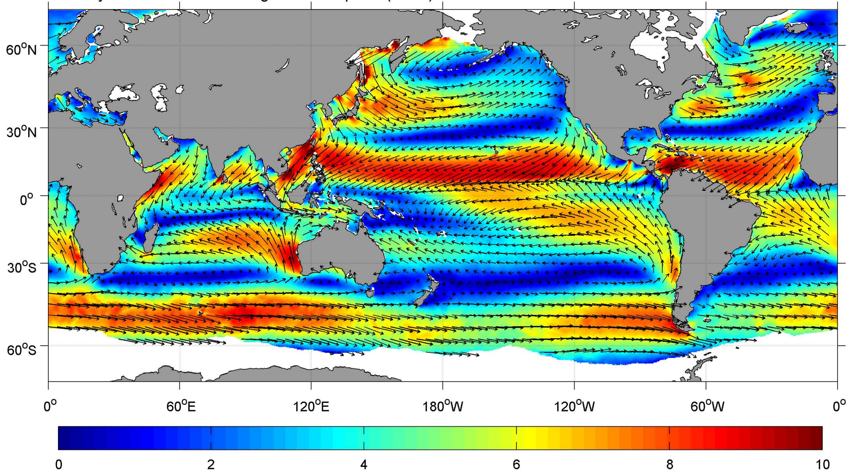
January SCOW Vector Averaged Wind Speed ( \text{m s}^{-1} ) and Direction
