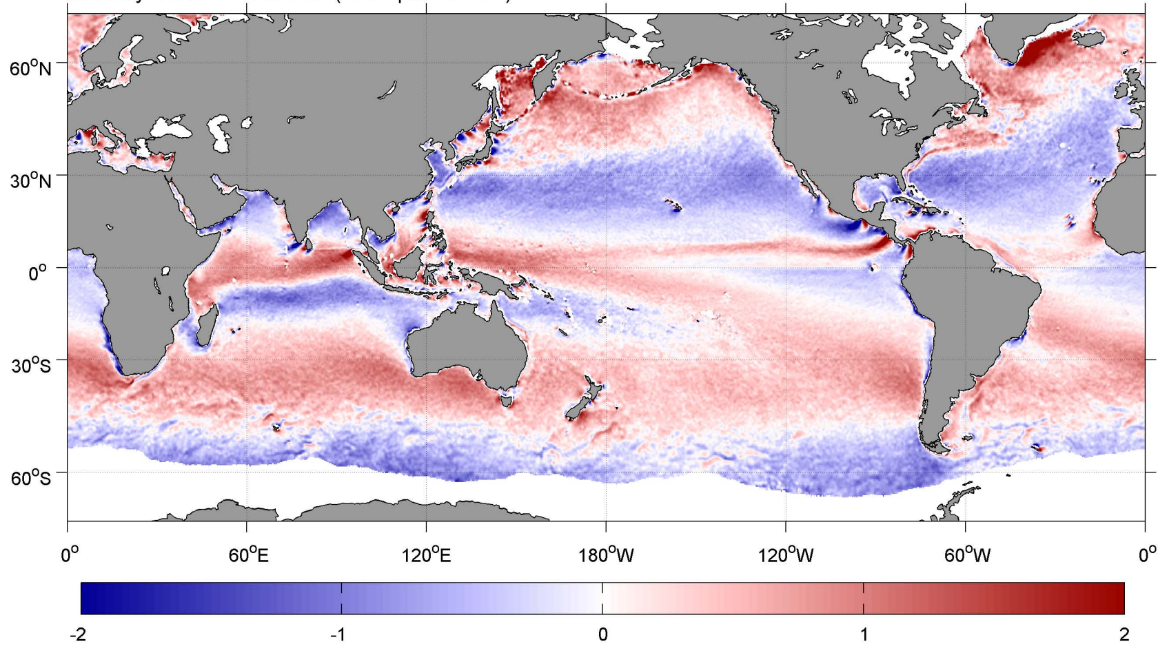
January SCOW Wind Curl ( \text{m s}^{-1} per 10^2 \text{ km} )
