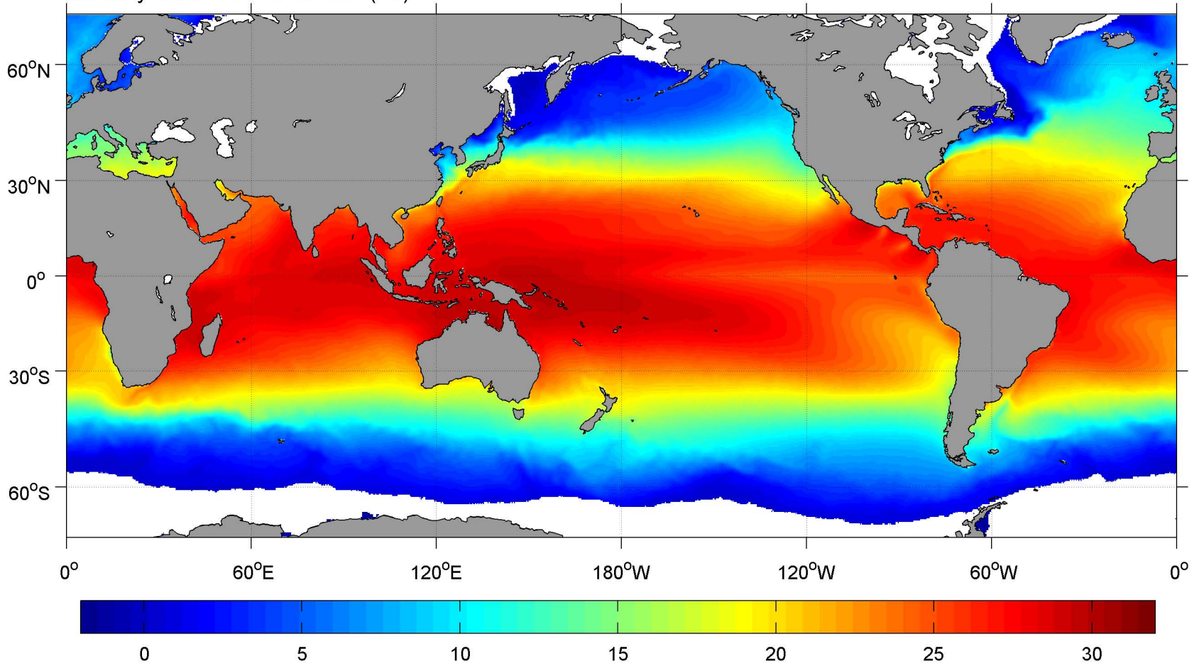
January SCOW AVHRR SST ( ^{\circ}\text{C} )
