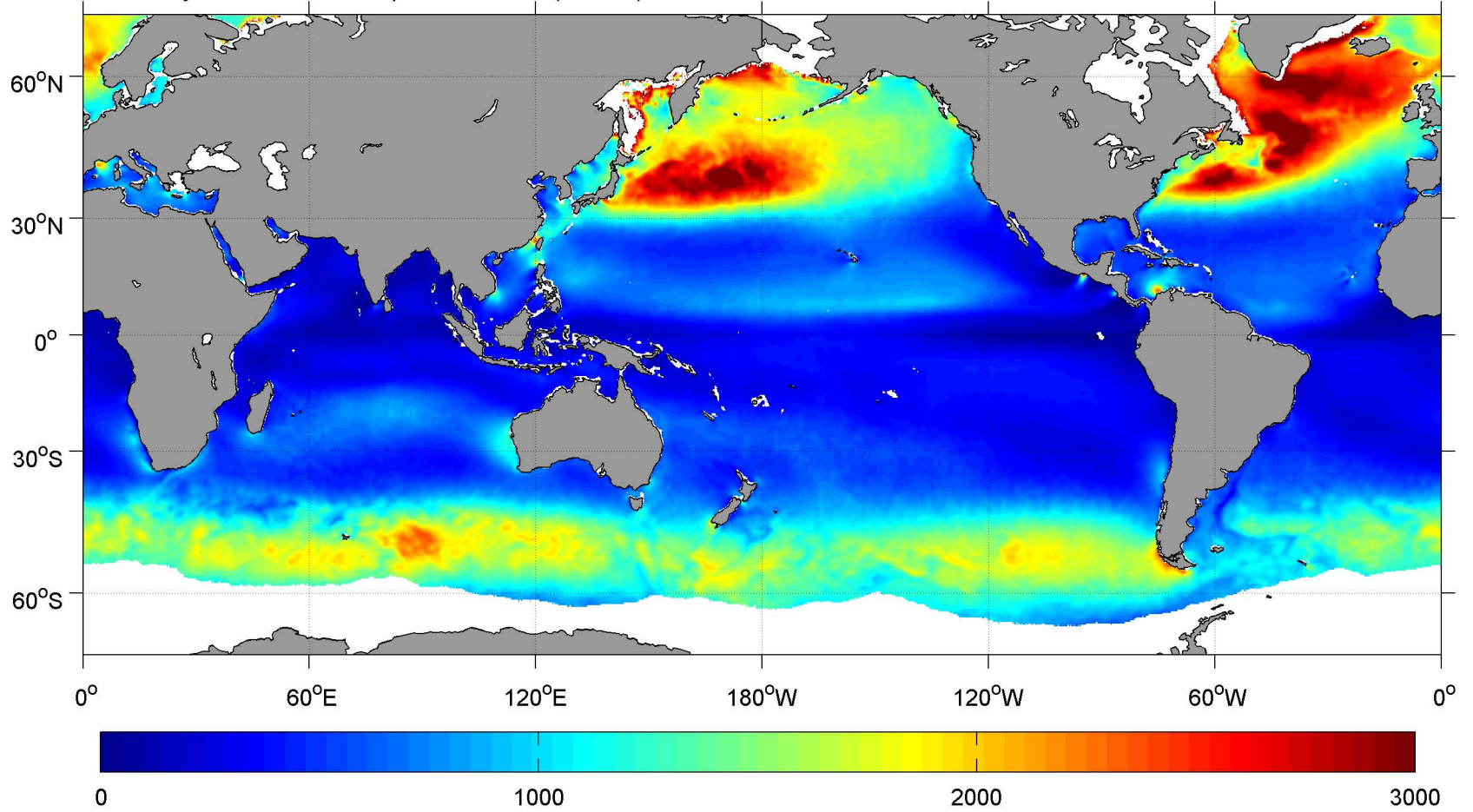
February SCOW Wind Speed Cubed ( \text{m}^3 \text{s}^{-3} )
