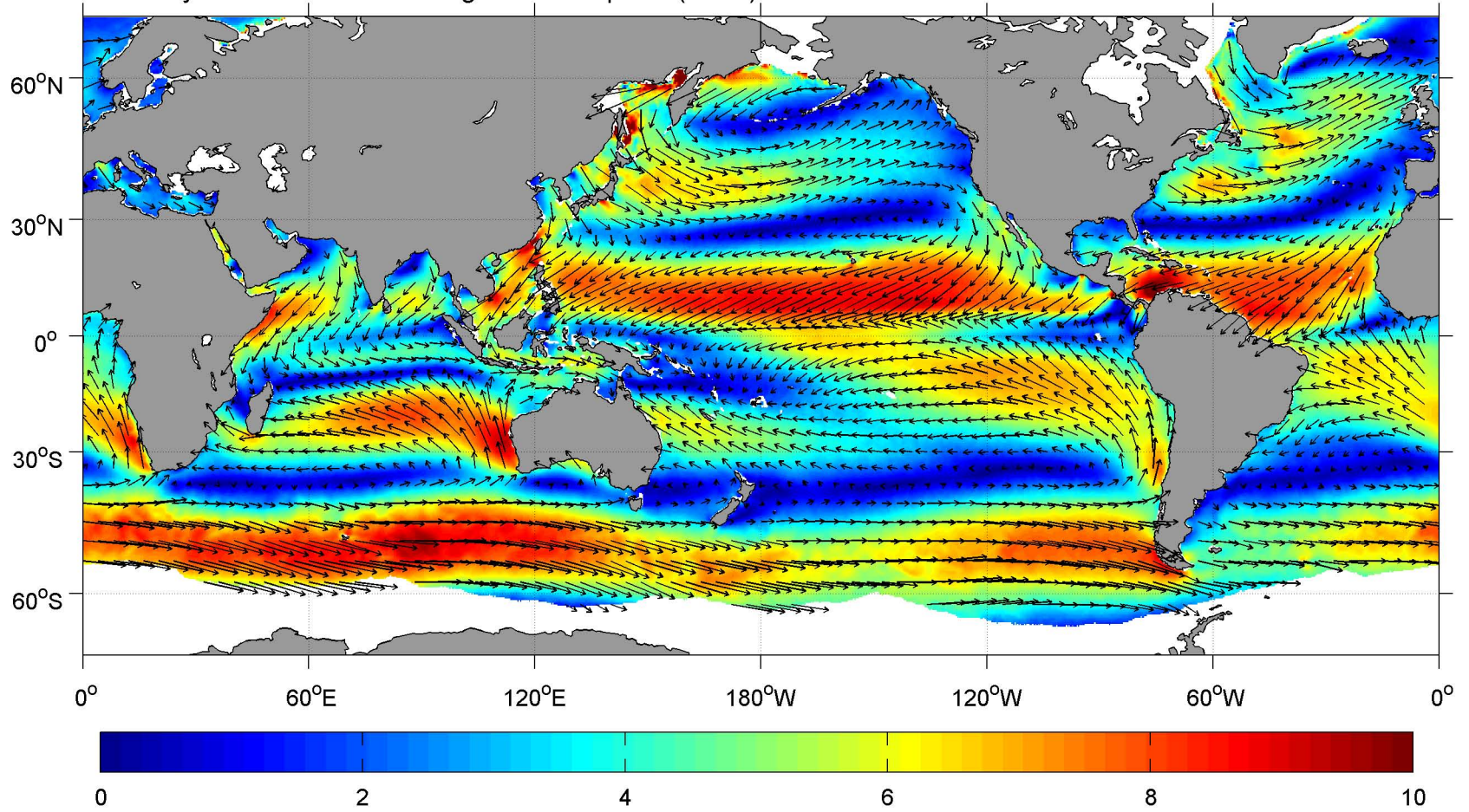
February SCOW Vector Averaged Wind Speed ( \text{m s}^{-1} ) and Direction
