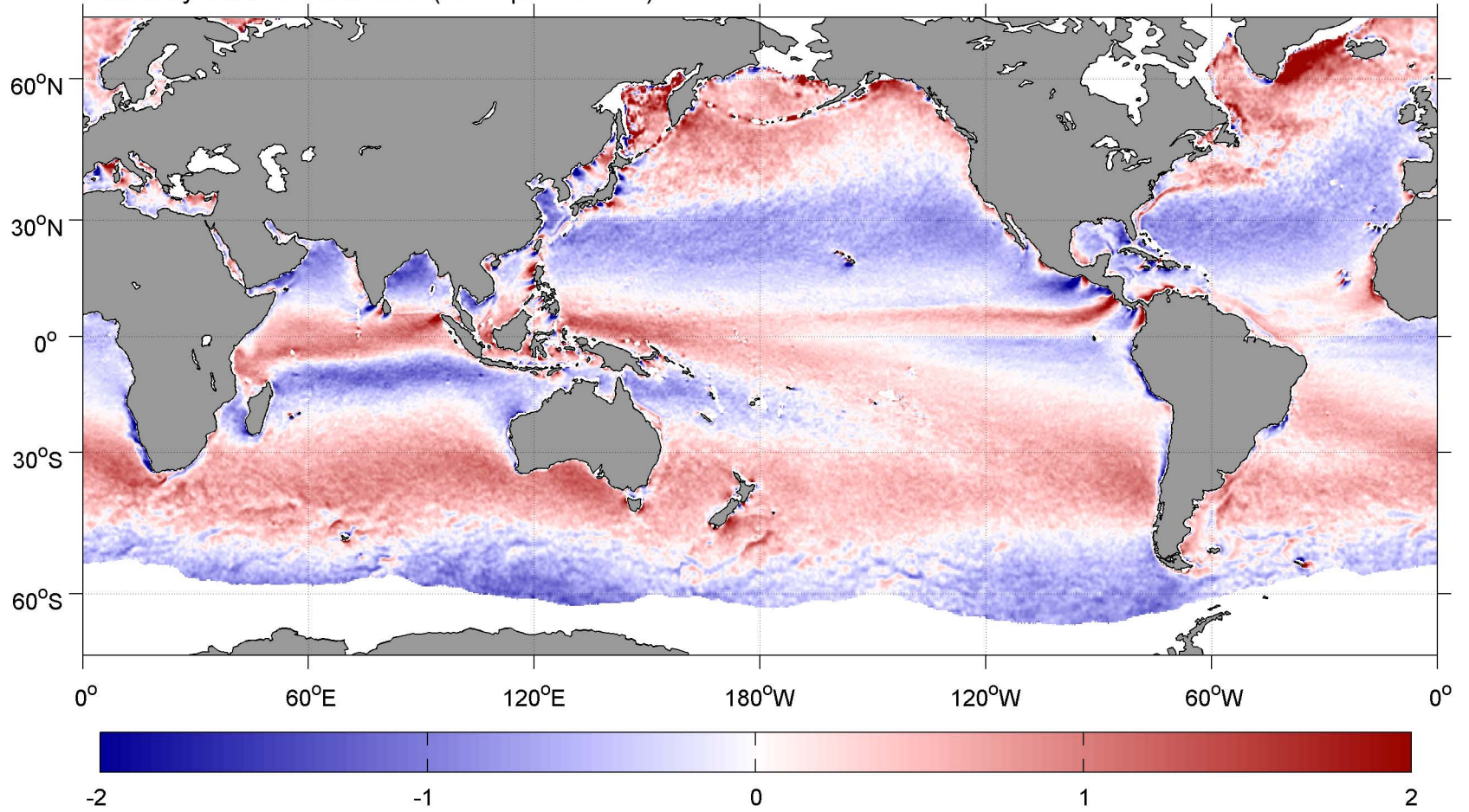
February SCOW Wind Curl ( \text{m s}^{-1} per 10^2 \text{ km} )
