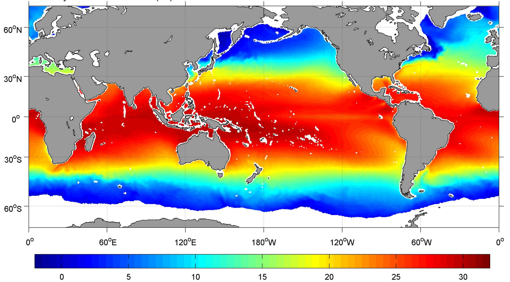
February SCOW AMSR SST ( ^{\circ}\text{C} )
