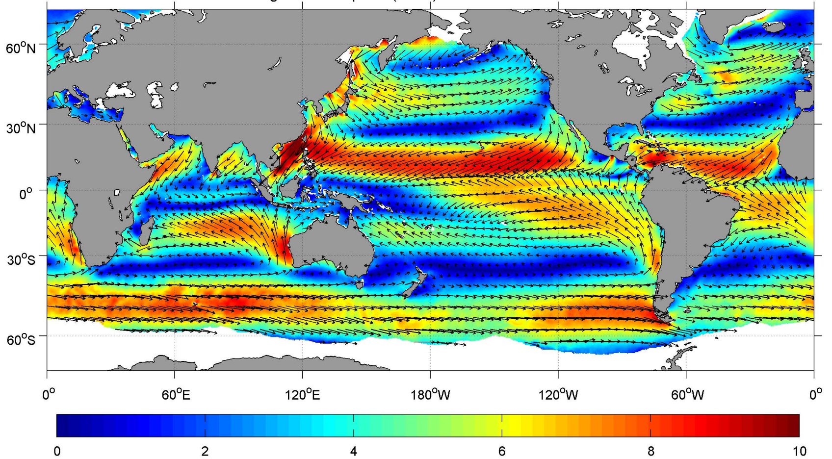
December SCOW Vector Averaged Wind Speed ( \text{m s}^{-1} ) and Direction
