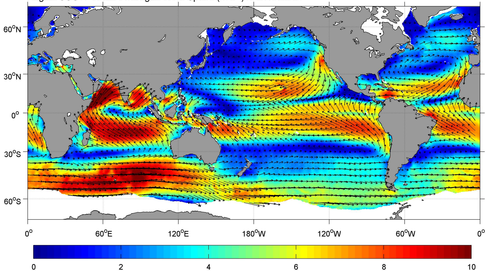
August SCOW Vector Averaged Wind Speed ( \text{m s}^{-1} ) and Direction
