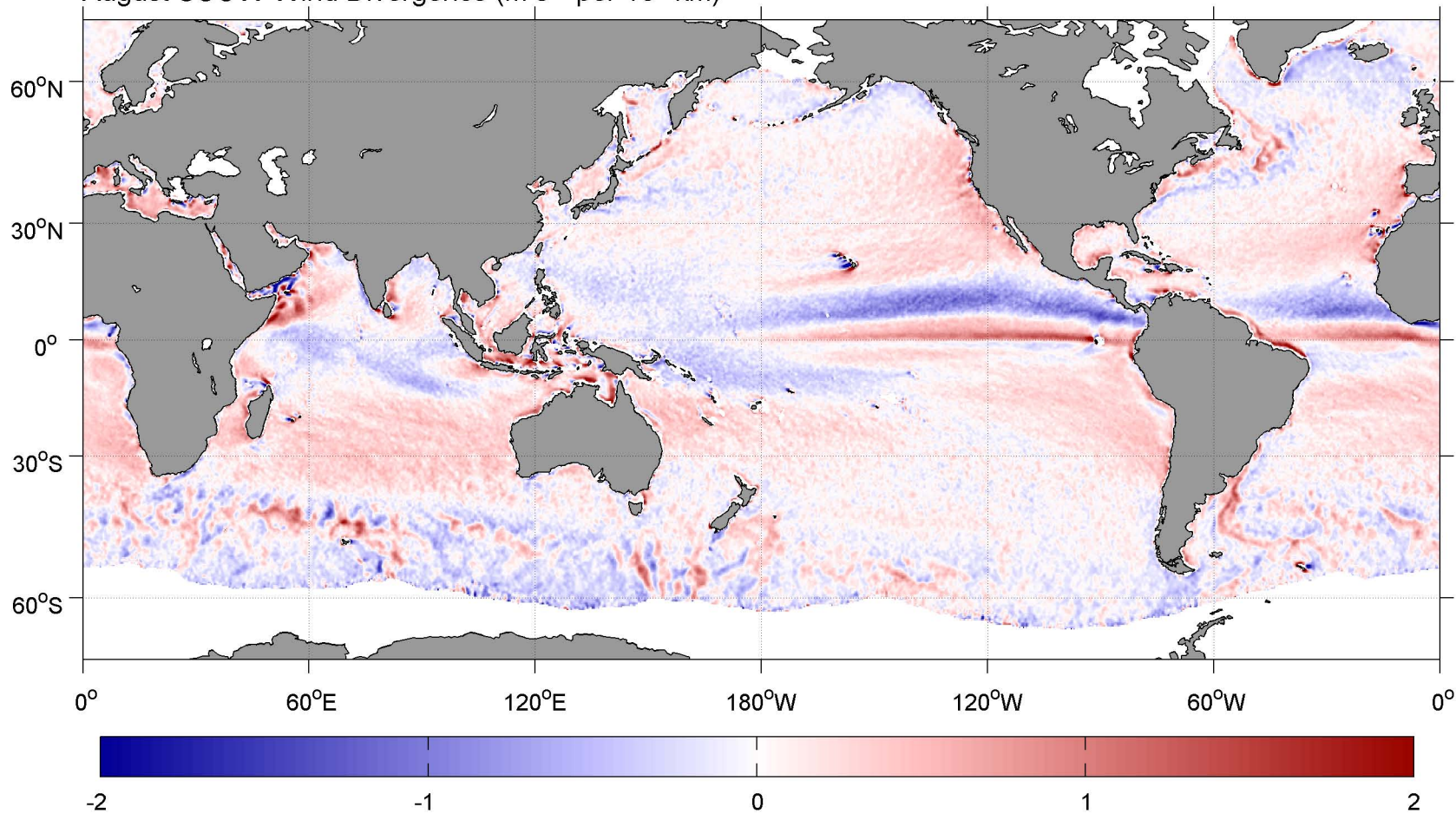
August SCOW Wind Divergence ( \text{m s}^{-1} per 10^2 \text{ km} )
