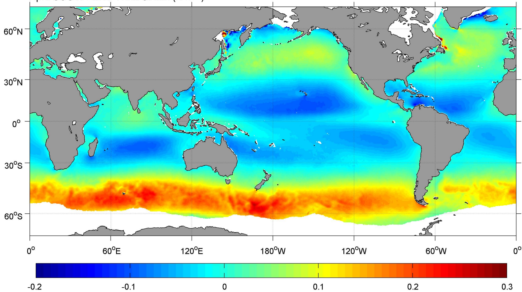
April SCOW Zonal Wind Stress ( \text{N m}^{-2} )
