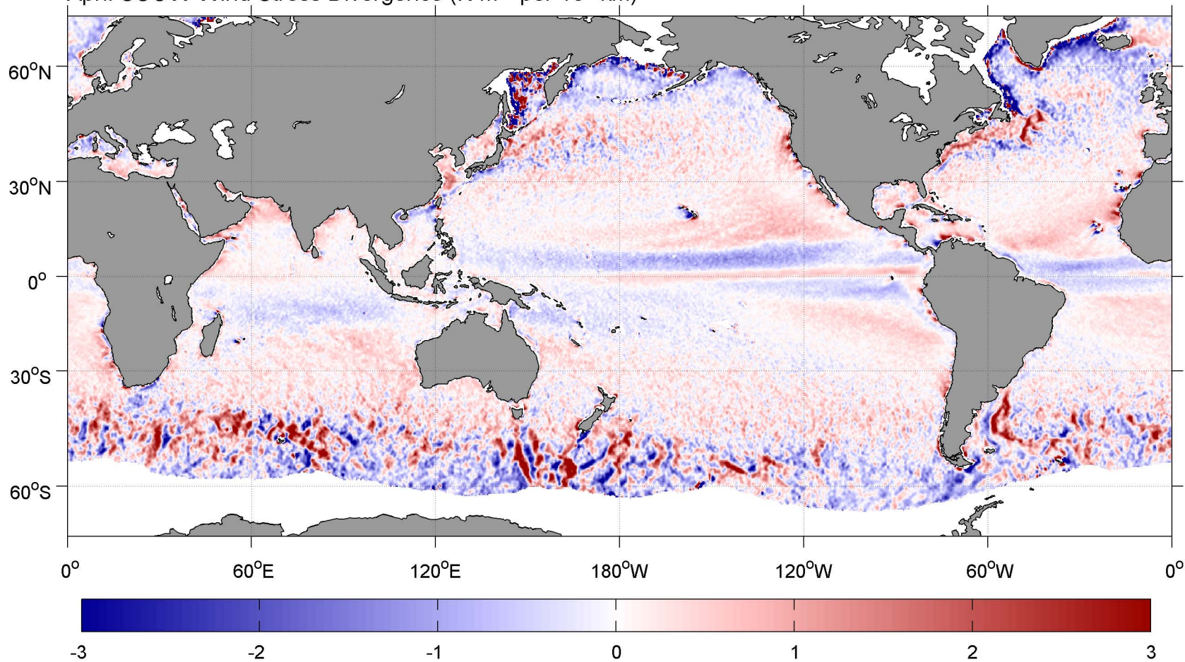
April SCOW Wind Stress Divergence ( \text{N m}^{-2} per 10^4 \text{ km}^2 )
