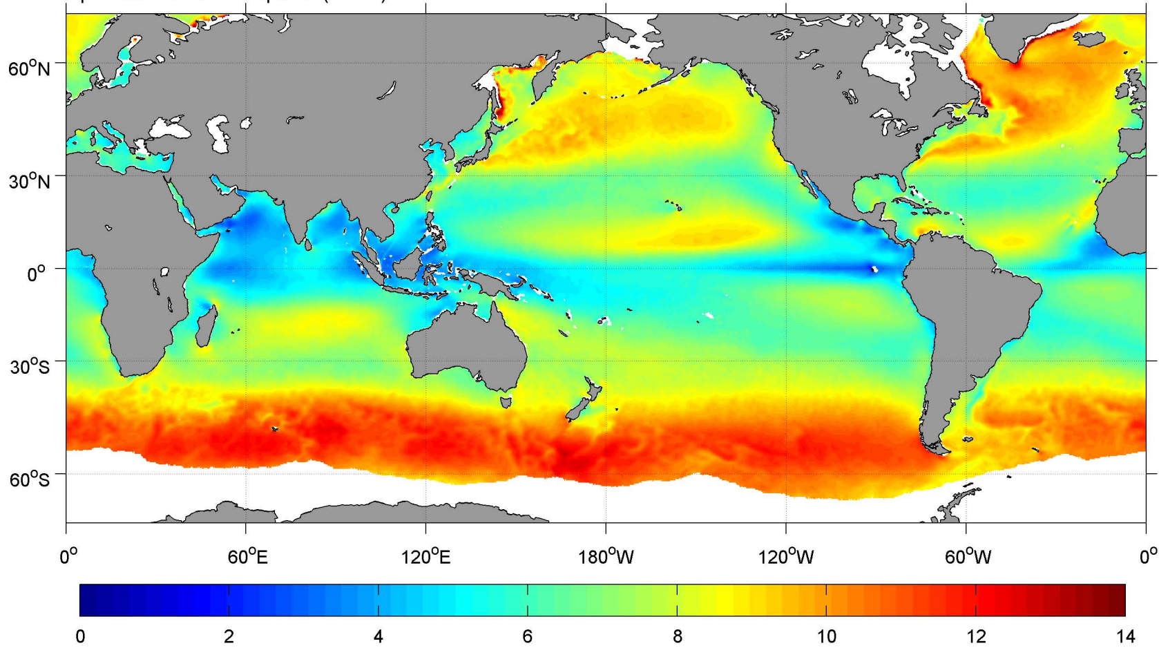
April SCOW Wind Speed ( \text{m s}^{-1} )
