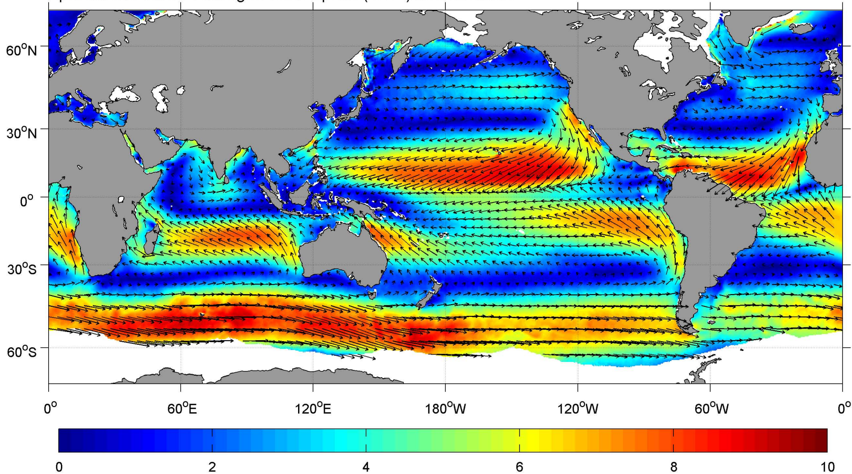
April SCOW Vector Averaged Wind Speed ( \text{m s}^{-1} ) and Direction
