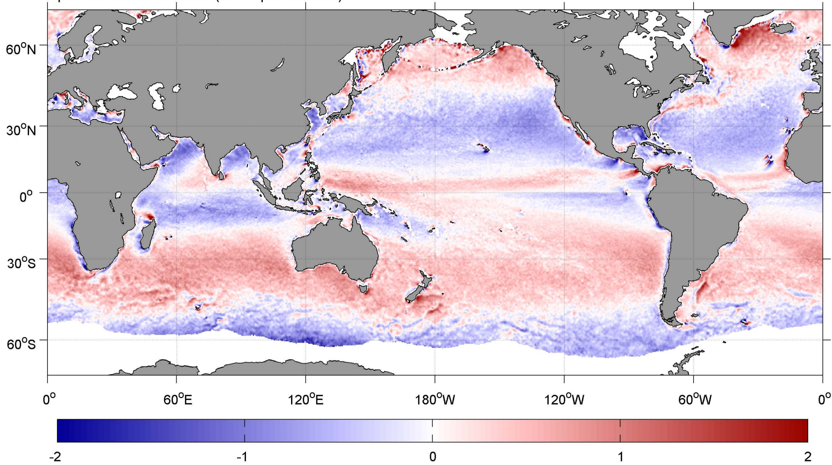
April SCOW Wind Curl ( \text{m s}^{-1} per 10^2 \text{ km} )
